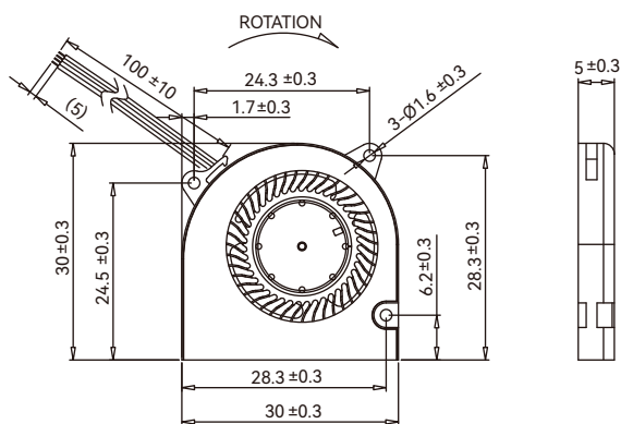
■ Dimensions Drawing (mm)
