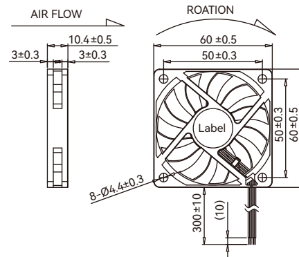
■ Dimensions Drawing (mm)
