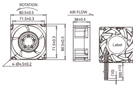
■ Dimensions Drawing (mm)
